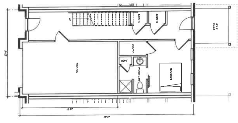
TOWNHOUSE - FIRST FLOOR / 1 SCALE: 1/4" = 1'-0"
