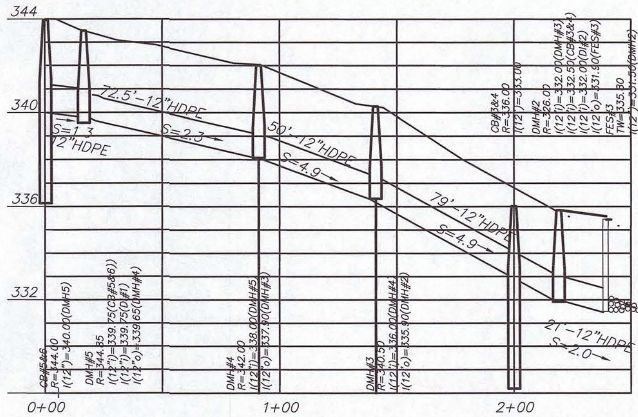
DRAINAGE PROFILE 3
