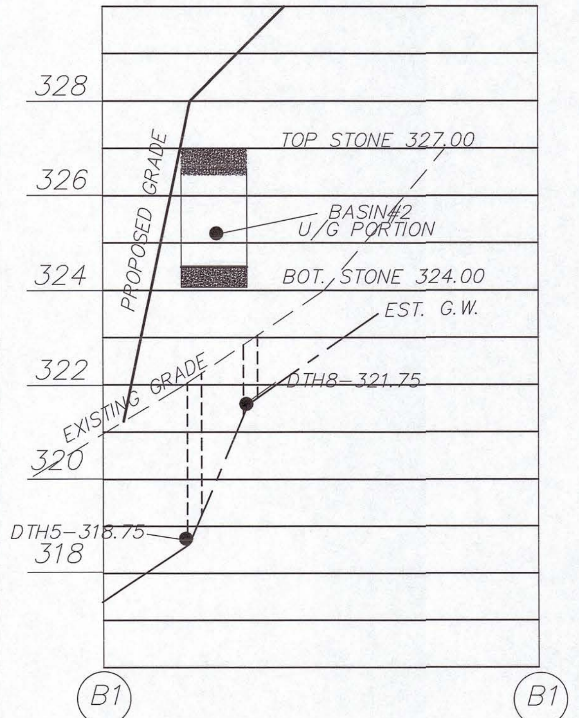
CROSS SECTION B1-B1
