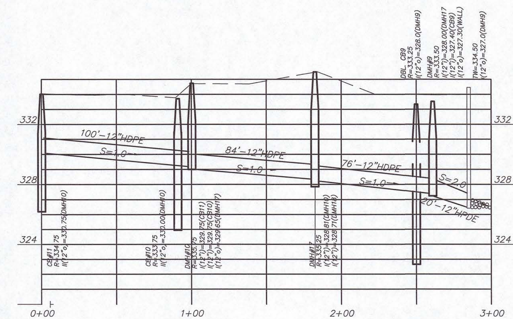
DRAINAGE PROFILE 1B
