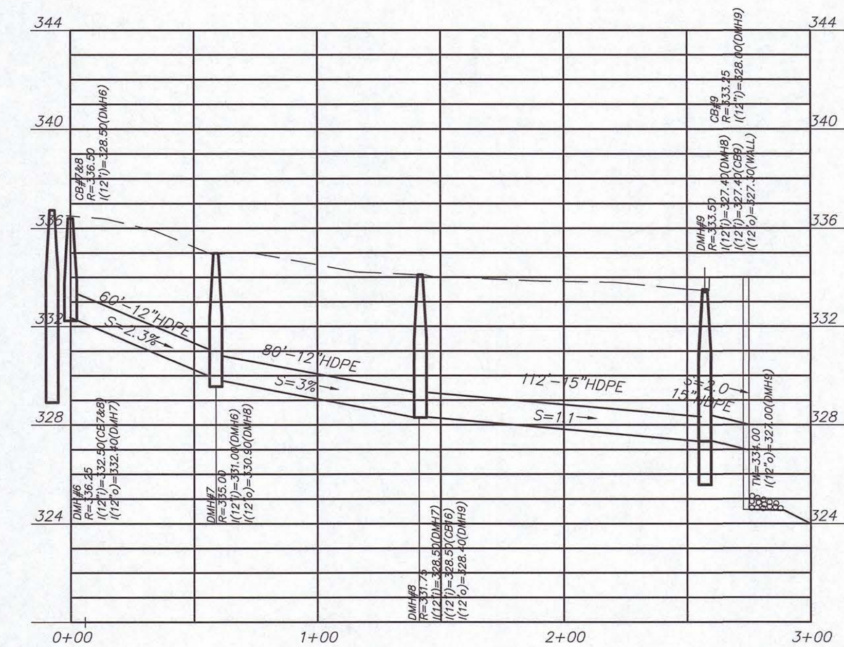
DRAINAGE PROFILE 1A
