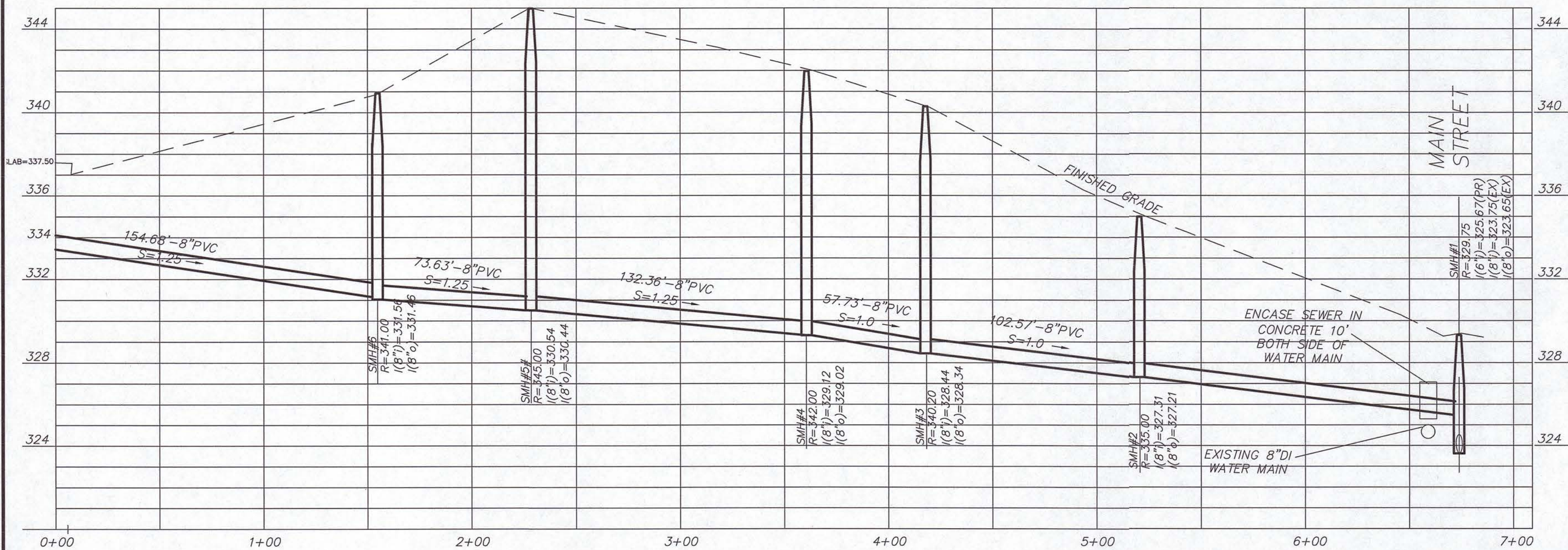
SEWER PROFILE
