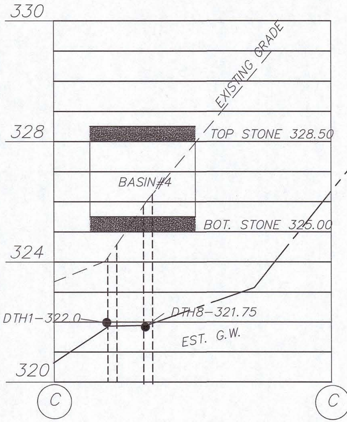
CROSS SECTION C-C
