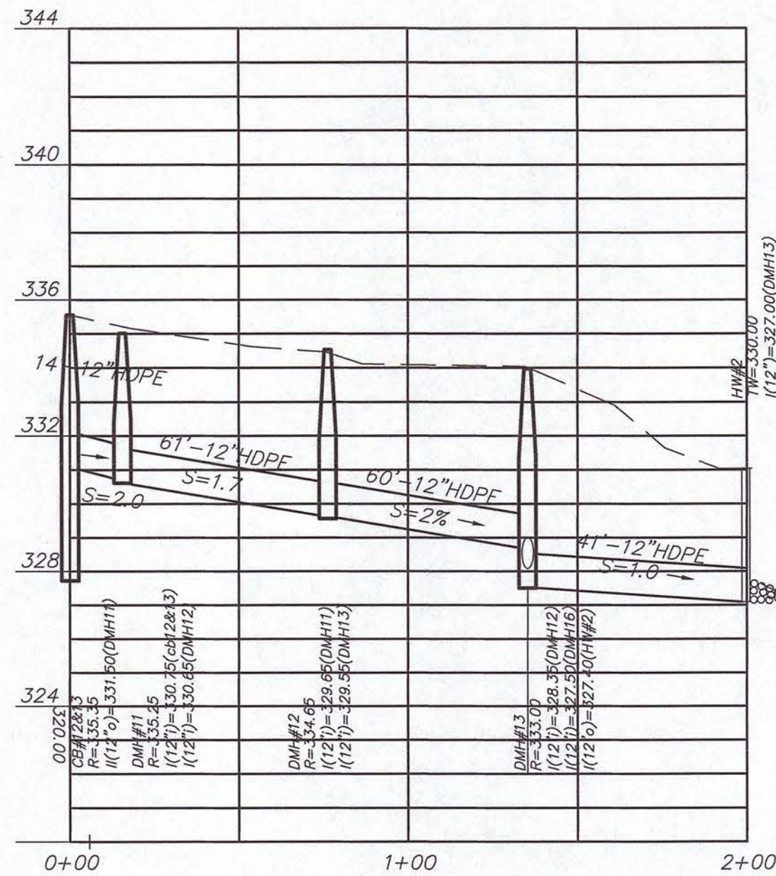
DRAINAGE PROFILE 2
